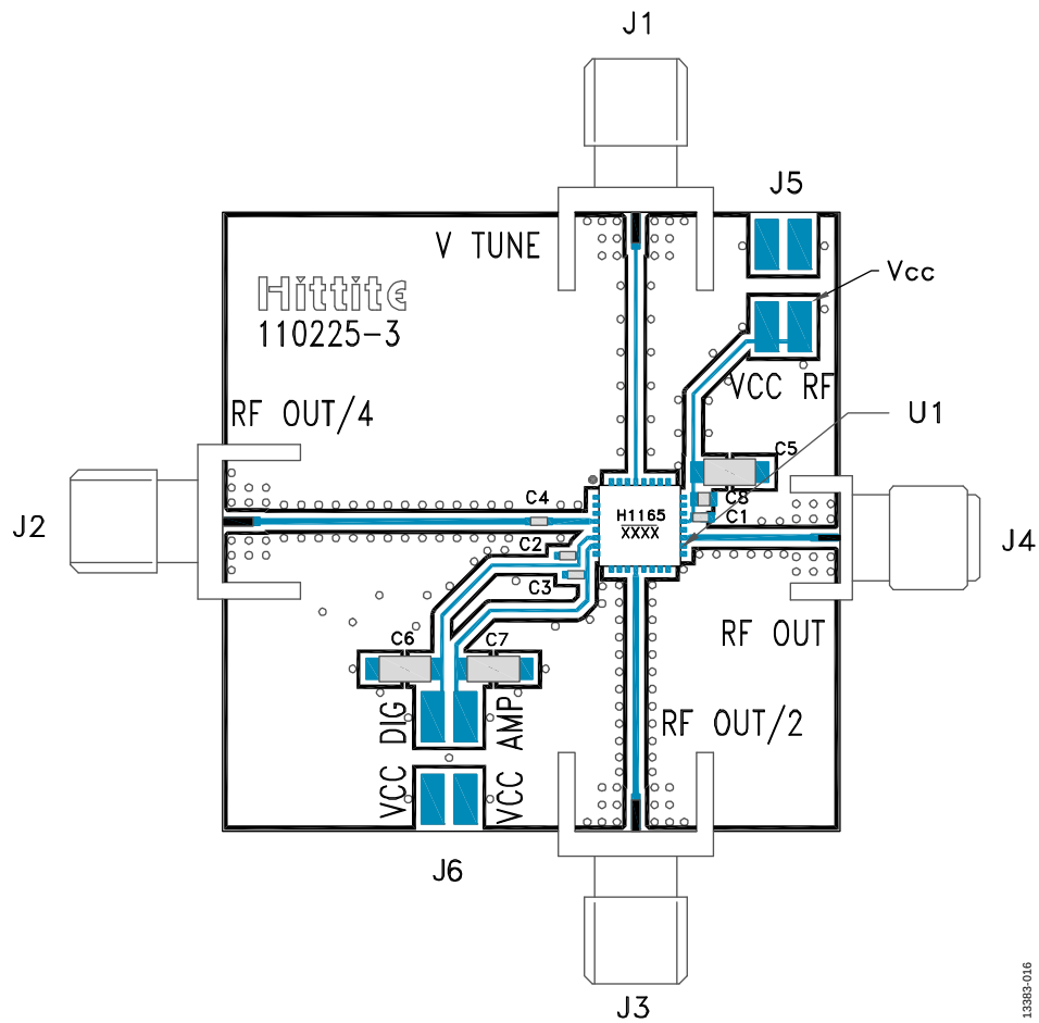
Figure 17. Evaluation Board
