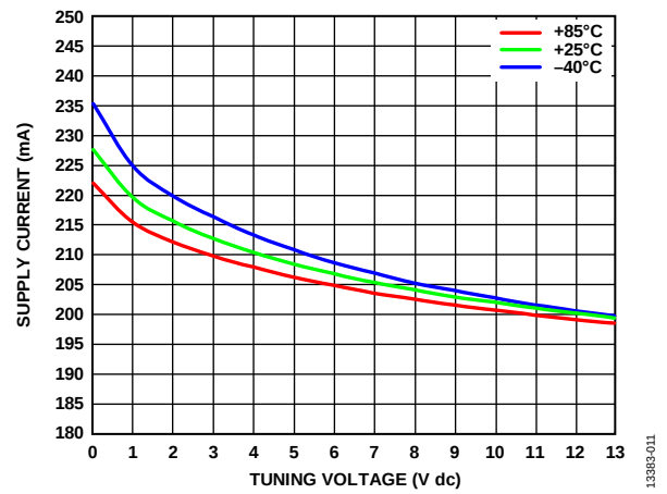
Figure 11. Supply Current vs. Tuning Voltage
