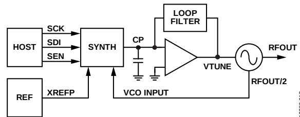
Figure 16. Typical Application Diagram
