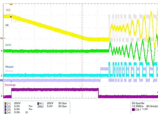
Figure 13. Initial Resonant Capacitor Discharge before Dedicated Startup Sequence is Placed
