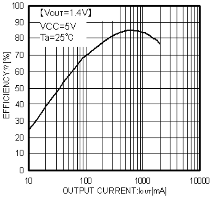
Fig.59 Efficiency
