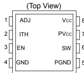
Fig.5 BD9120HFN
