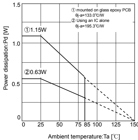
Fig.94 Thermal derating curve (HSO8)
