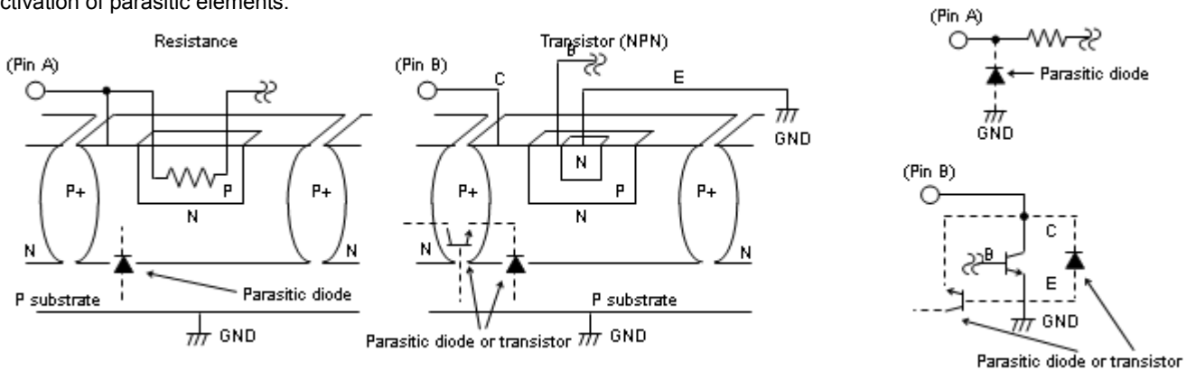
Fig.106 Simplified structure of monolithic IC
