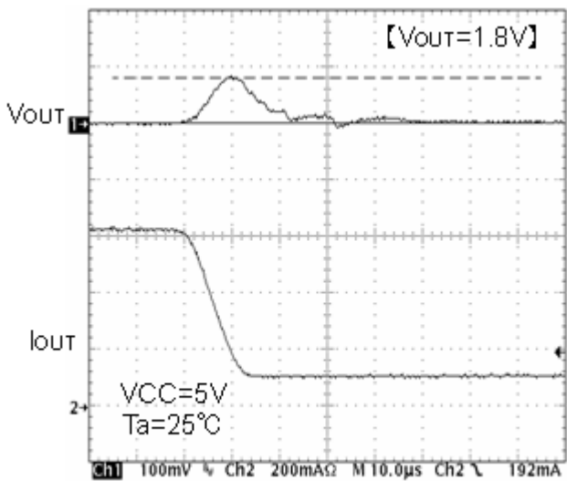
Fig.24 Transient response Io=600→100mA(10µs)
