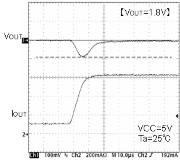
Fig. 23 Transient response Io=100→600mA(10µs)
