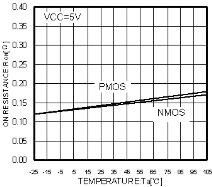
Fig.61 T_a - R_{onn} , R_{onp}
