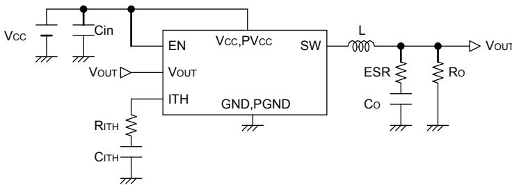
Fig.101 Typical application
