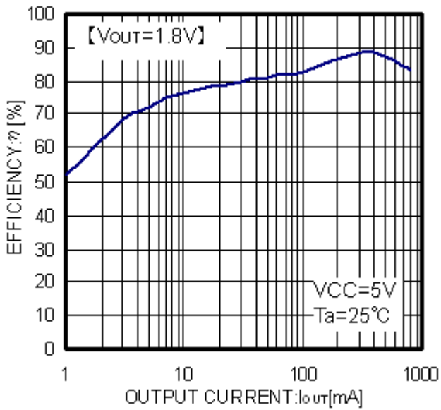
Fig.14 Efficiency
