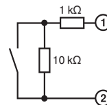
Figure 8 Switch contact with resistance circuit
