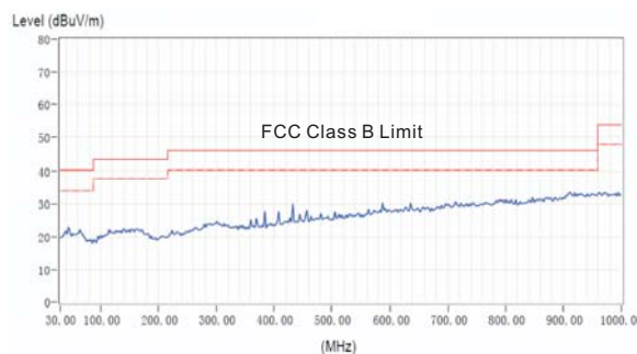
Radiated Emissions
