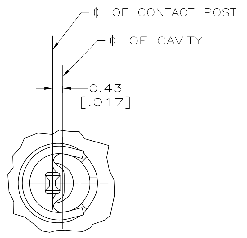
VIEW B-B SCALE 10:1 5 PLC
