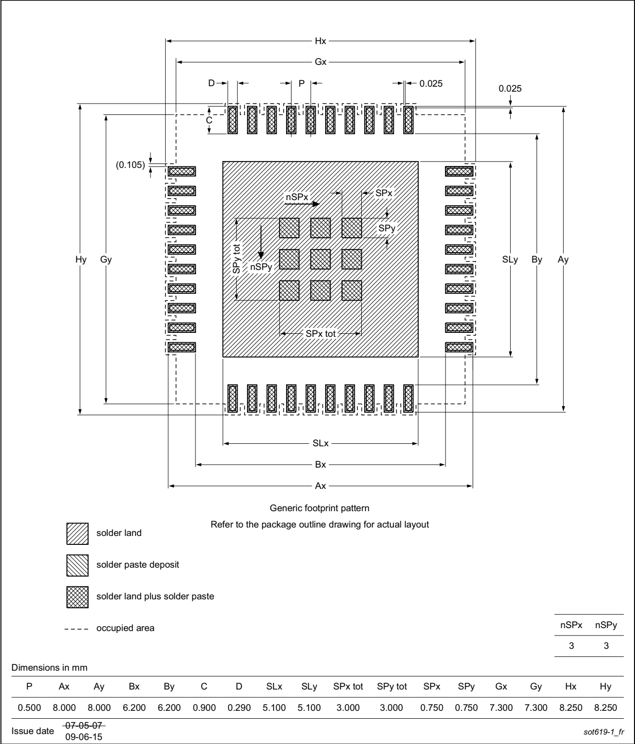
Footprint information for reflow soldering of HVQFN48 package SOT619-1
