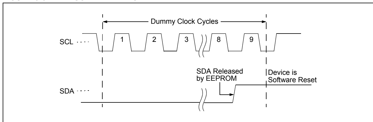
FIGURE 5-3: SOFTWARE RESET
