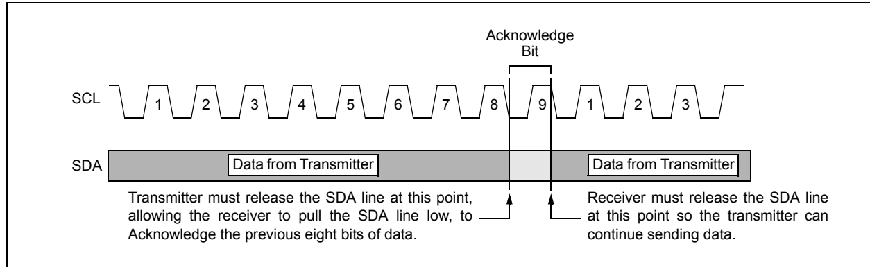
FIGURE 5-2: ACKNOWLEDGE TIMING
