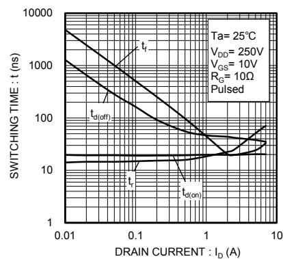
Fig.12 Switching Characteristics
