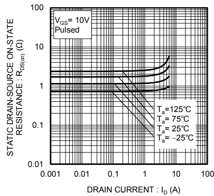
Fig.5 Static Drain-Source On-State Resistance vs. Drain Current
