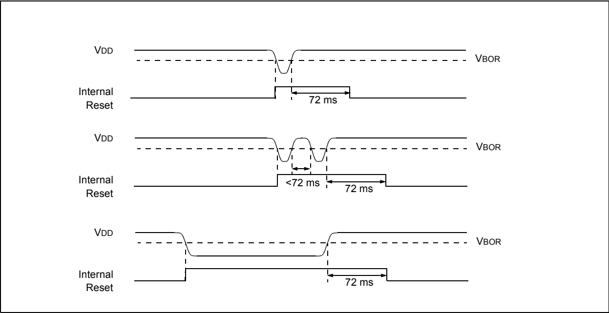
FIGURE 9-6: BROWN-OUT SITUATIONS (PWRT TE = 0)
