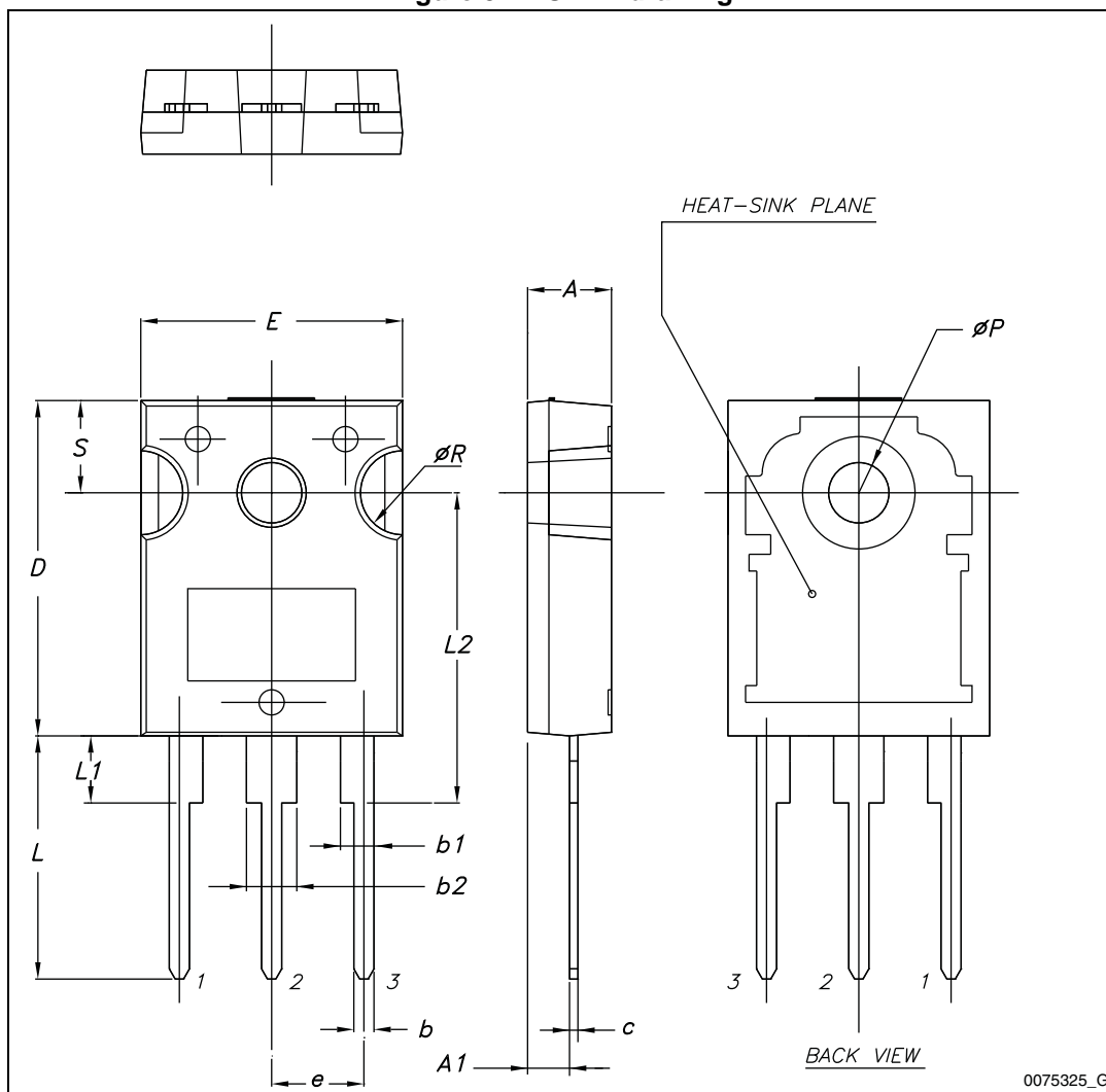
Figure 32. TO-247 drawing
