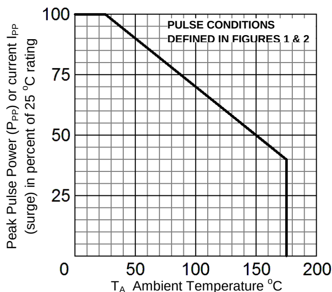
FIGURE 3 DERATING CURVE
