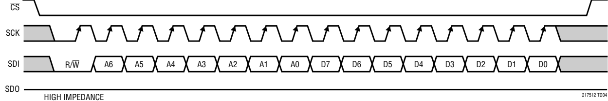
SPI Port Timing (Write Mode)
