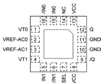
16-Pin QFN
