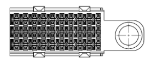
Part Number 120949-1 60 Position Receptacle with Guide Module
