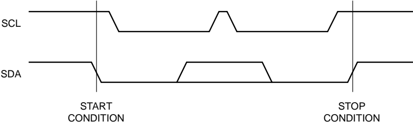
Figure 5. START/STOP Condition
