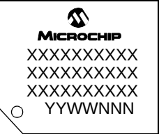
44-Lead TQFP
