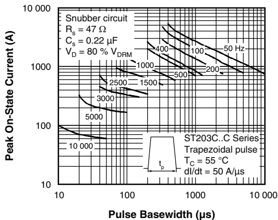
Fig. 14 - Frequency Characteristics
