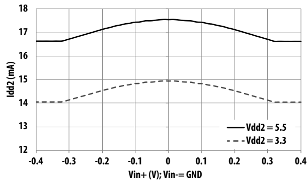
Figure 20. I_{DD2} vs. Input Voltage V_{IN}
