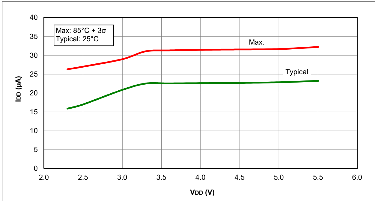
FIGURE 31-8: I_{DD} , EXTERNAL CLOCK (ECL), LOW-POWER MODE, F_{osc} = 32\text{ kHz} , PIC12F1840 ONLY
