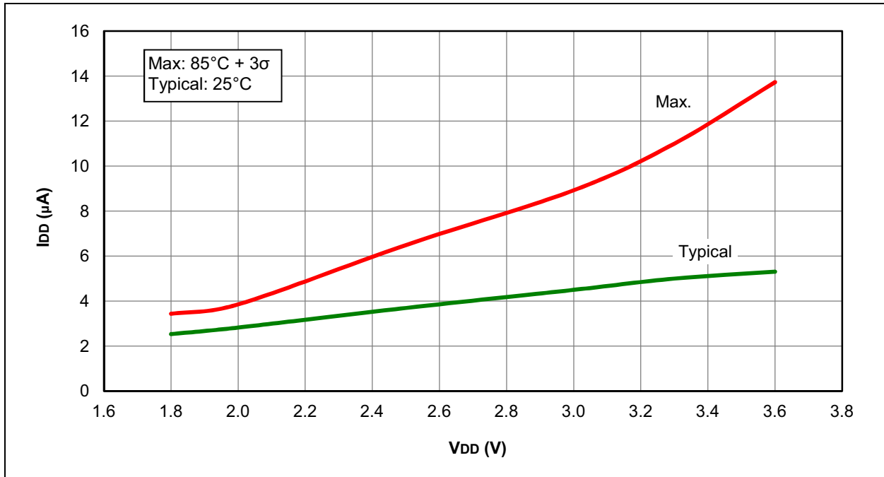
FIGURE 31-7: I_{DD} , EXTERNAL CLOCK (ECL), LOW-POWER MODE, F_{osc} = 32\text{ kHz} , PIC12LF1840 ONLY
