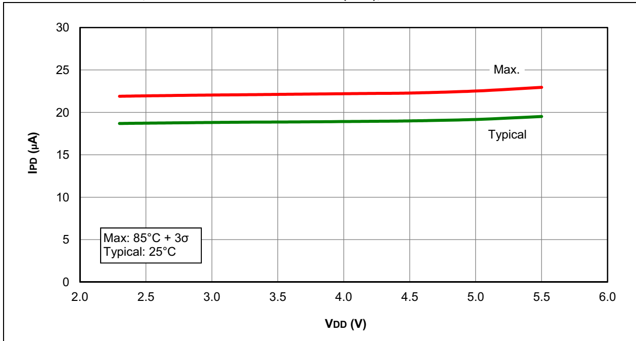
FIGURE 31-36: I_{PD} , FIXED VOLTAGE REFERENCE (FVR), PIC12F1840 ONLY
