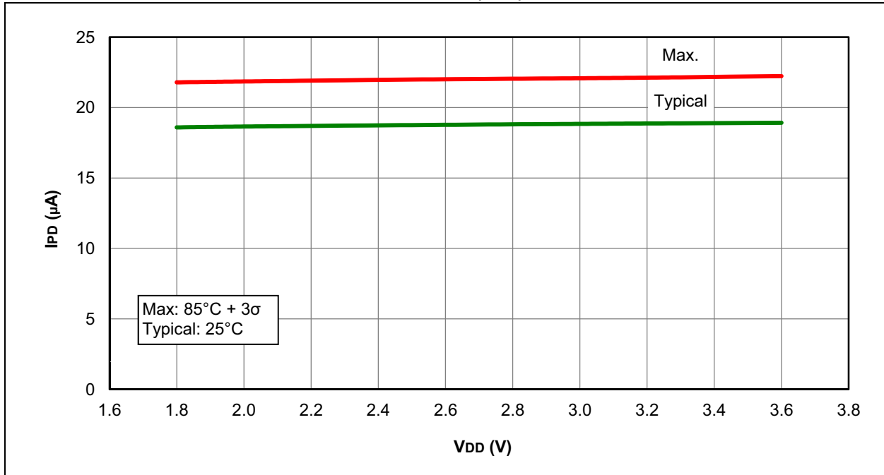
FIGURE 31-35: I_{PD} , FIXED VOLTAGE REFERENCE (FVR), PIC12LF1840 ONLY
