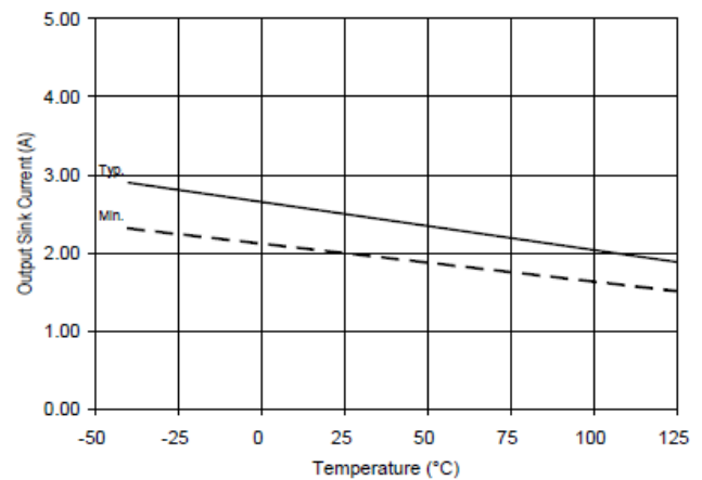
Figure 25A. Output Sink Current vs. Temperature
