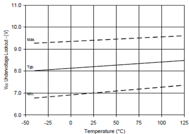
Figure 23. V_{CC} Undervoltage (-) vs. Temperature
