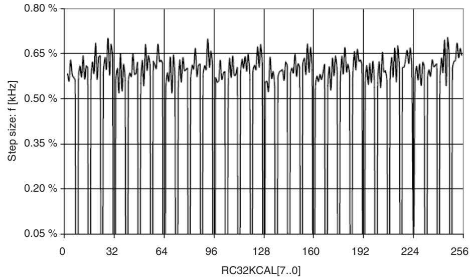
Figure 35-37. Internal 32.768 kHz Oscillator Calibration Step Size
