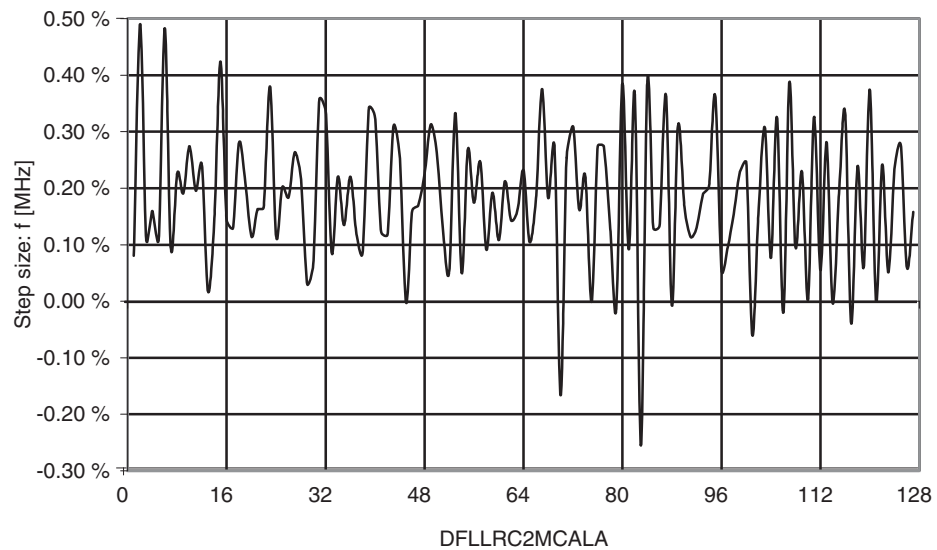
Figure 35-38. Internal 2 MHz Oscillator CALA Calibration Step Size
