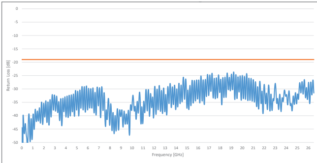
Return Loss SUCOFLEX 526S with two straight PC3.5 connectors
