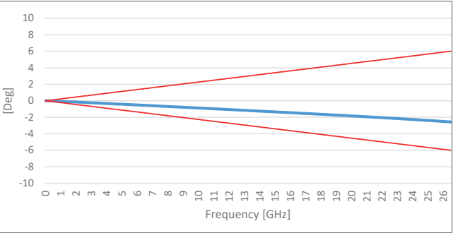
Phase vs. stability vs. flexure
