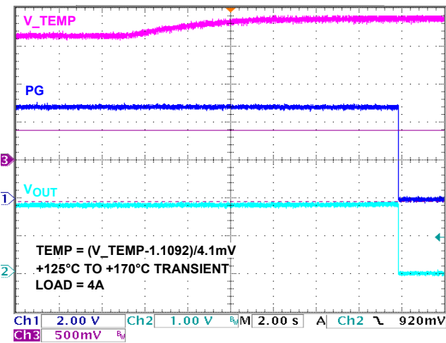
FIGURE 42. OVER-TEMPERATURE PROTECTION
