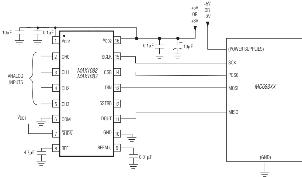
Figure 16. QSPI Connections, External Reference
