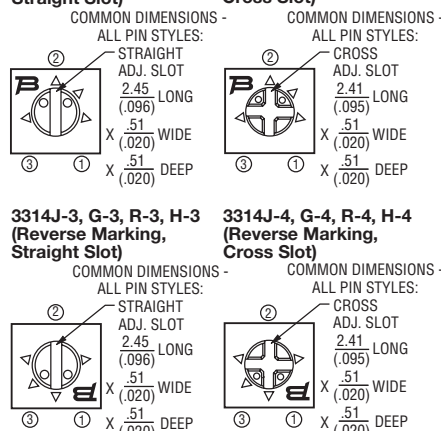
3314J-1, G-1, R-1, H-1 (Bourns Marking, Straight Slot)
