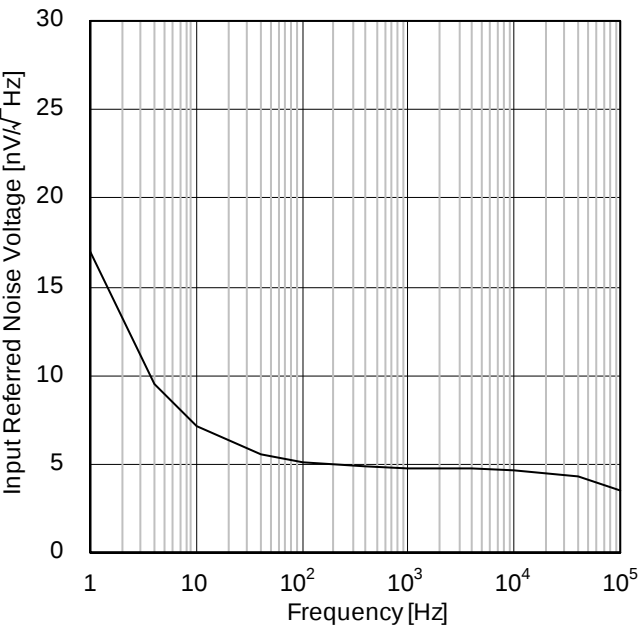
Figure 19. Input Referred Noise Voltage vs Frequency (VCC/VEE=±15V, T A =25°C, A v =40dB)
