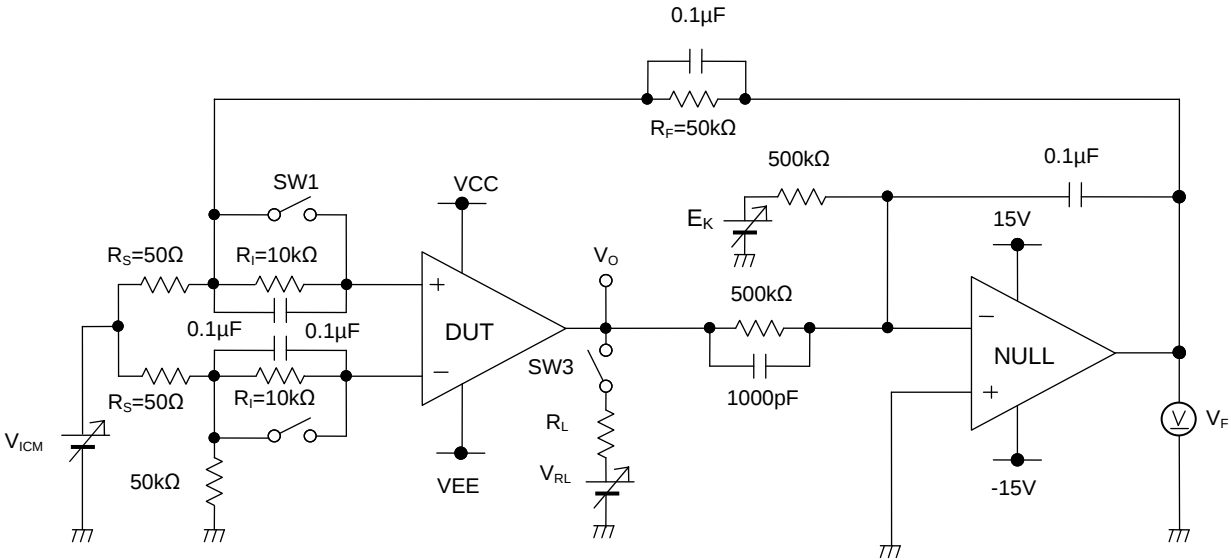
Figure21. Test Circuit 1
