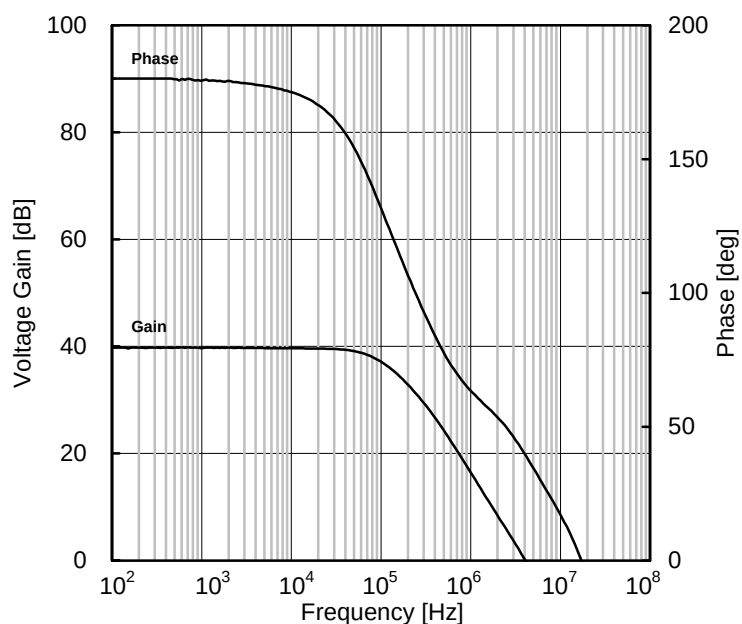
Figure 17. Voltage Gain • Phase vs Frequency (VCC/VEE=±15V, R L =2kΩ)
