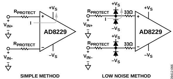
Figure 61. Protection for Voltages Beyond the Rails
