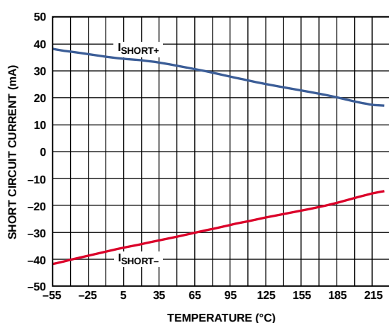
Figure 28. Short-Circuit Current vs. Temperature, G = 1
