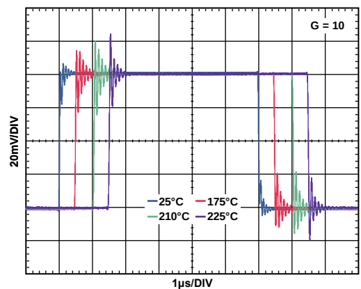
Figure 46. Small Signal Response, G = 10 , R_L = 10 k \Omega , C_L = 100 pF
