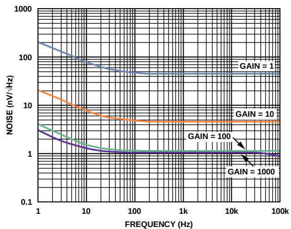
Figure 38. Voltage Noise Spectral Density vs. Frequency
