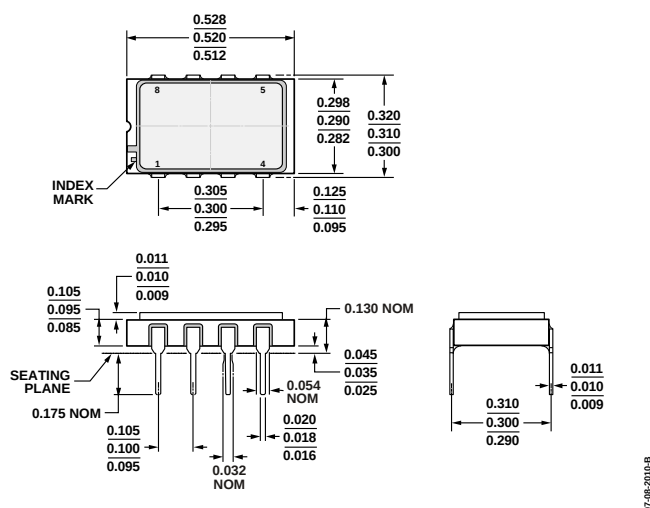
Figure 65. 8-Lead Side-Brazed Ceramic Dual In-Line Package [SBDIP] (D-8-1)
