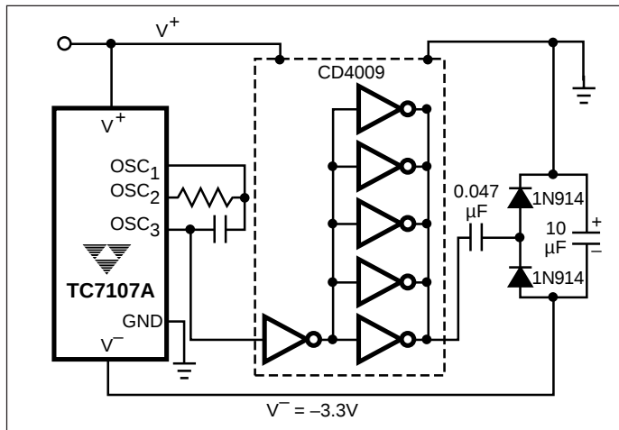
Figure 12. Generating Negative Supply From +5\text{V}
