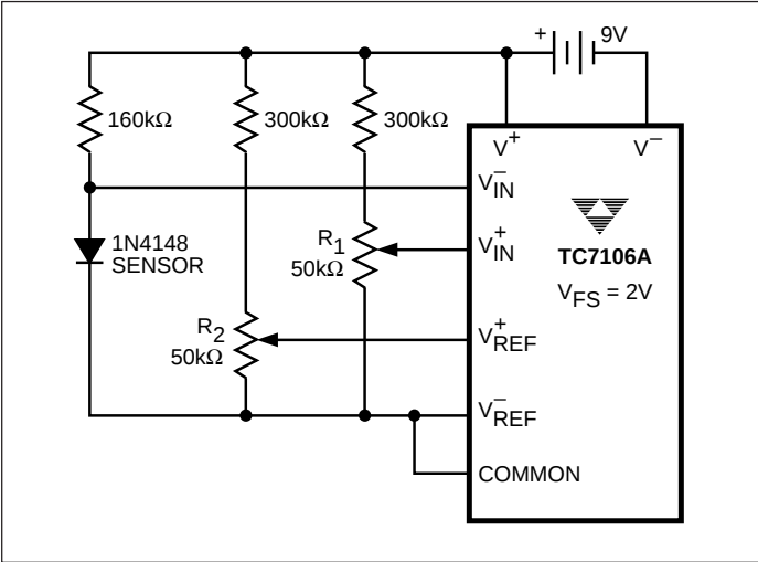
Figure 19. Temperature Sensor
