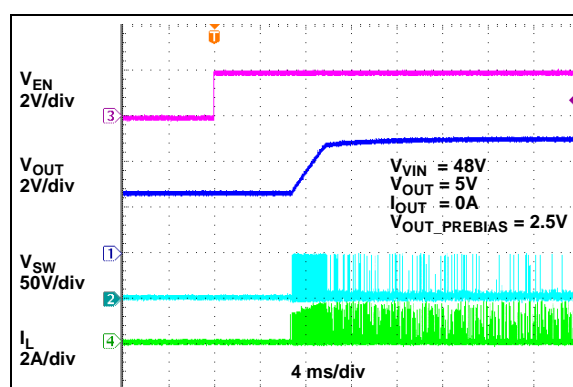
FIGURE 2-41: Enable Turn-On with Prebiased Output (HLL Mode).
