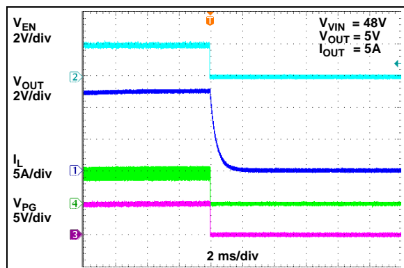
FIGURE 2-37: Enable Turn-Off Delay.
