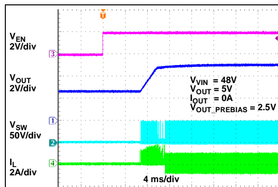
FIGURE 2-40: Enable Turn-On with Prebiased Output (CCM Mode).
