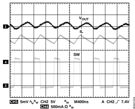
Figure 26. Steady State at Heavy Load, f_{SW} = 1.4 MHz , I_{OUT} = 1 A
