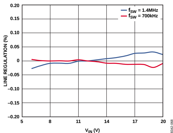
Figure 13. Line Regulation, V_{OUT} = 3.3\text{ V} , I_{OUT} = 500\text{ mA}
