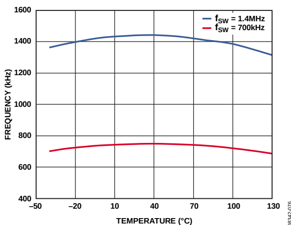
Figure 14. Frequency vs. Temperature
