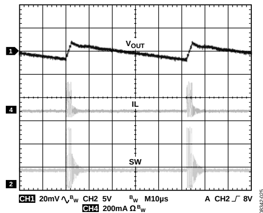
Figure 27. Steady State at Light Load, f_{SW} = 1.4 MHz , I_{OUT} = 40 mA
