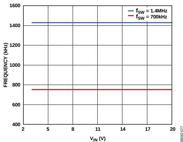
Figure 15. Frequency vs. V_{IN}
