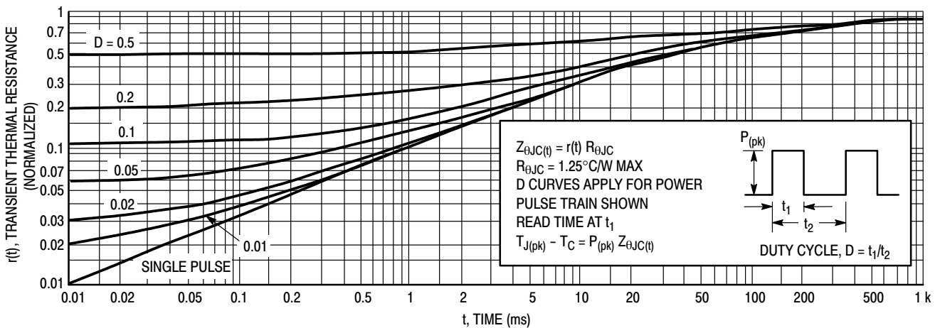
Figure 11. Typical Thermal Response [Z θJC (t)]
