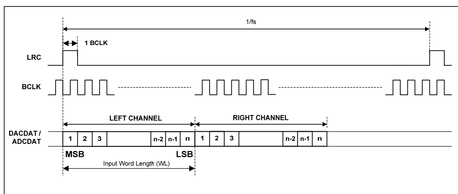
Figure 39 DSP/PCM Mode Audio Interface (mode B, LRP=1)
