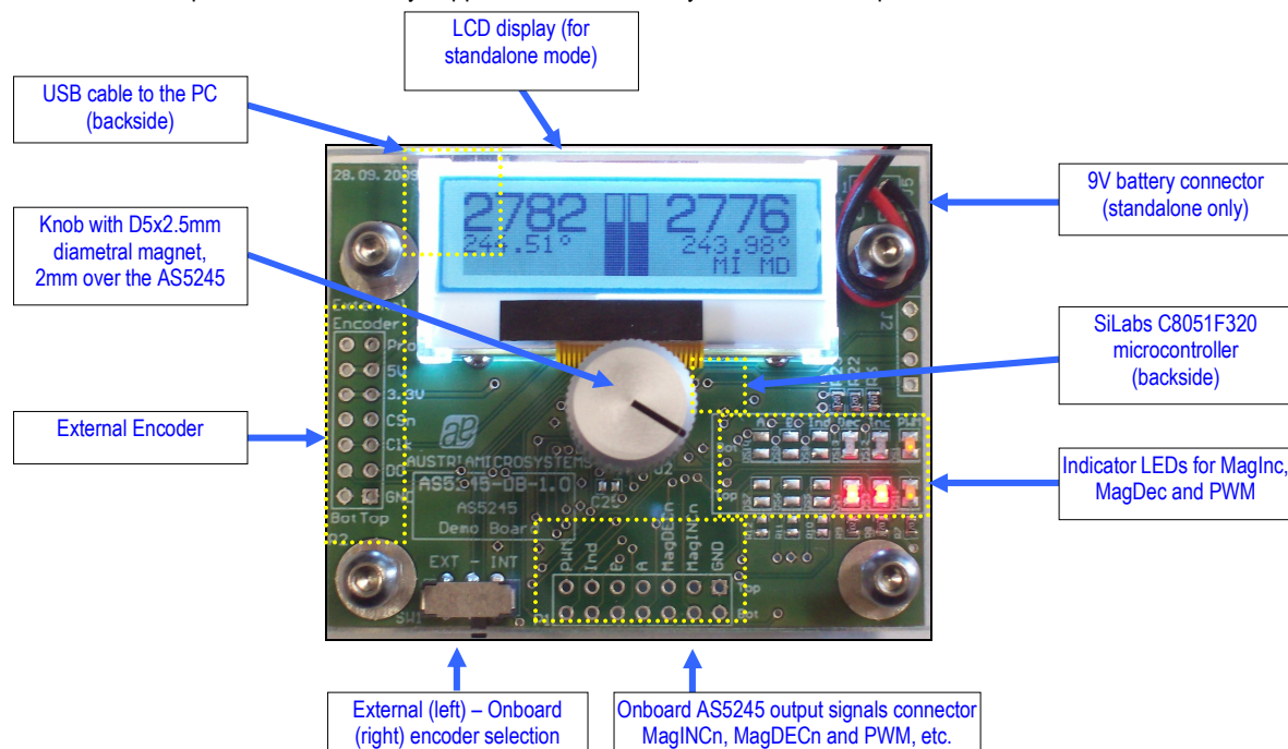
Figure 1: AS5245 Demoboard hardware with mounted magnet knob
