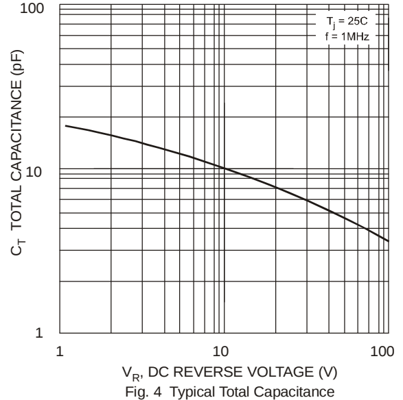
V_R , DC REVERSE VOLTAGE (V) Fig. 4 Typical Total Capacitance
