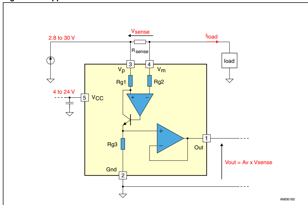
Figure 1. Application schematics
