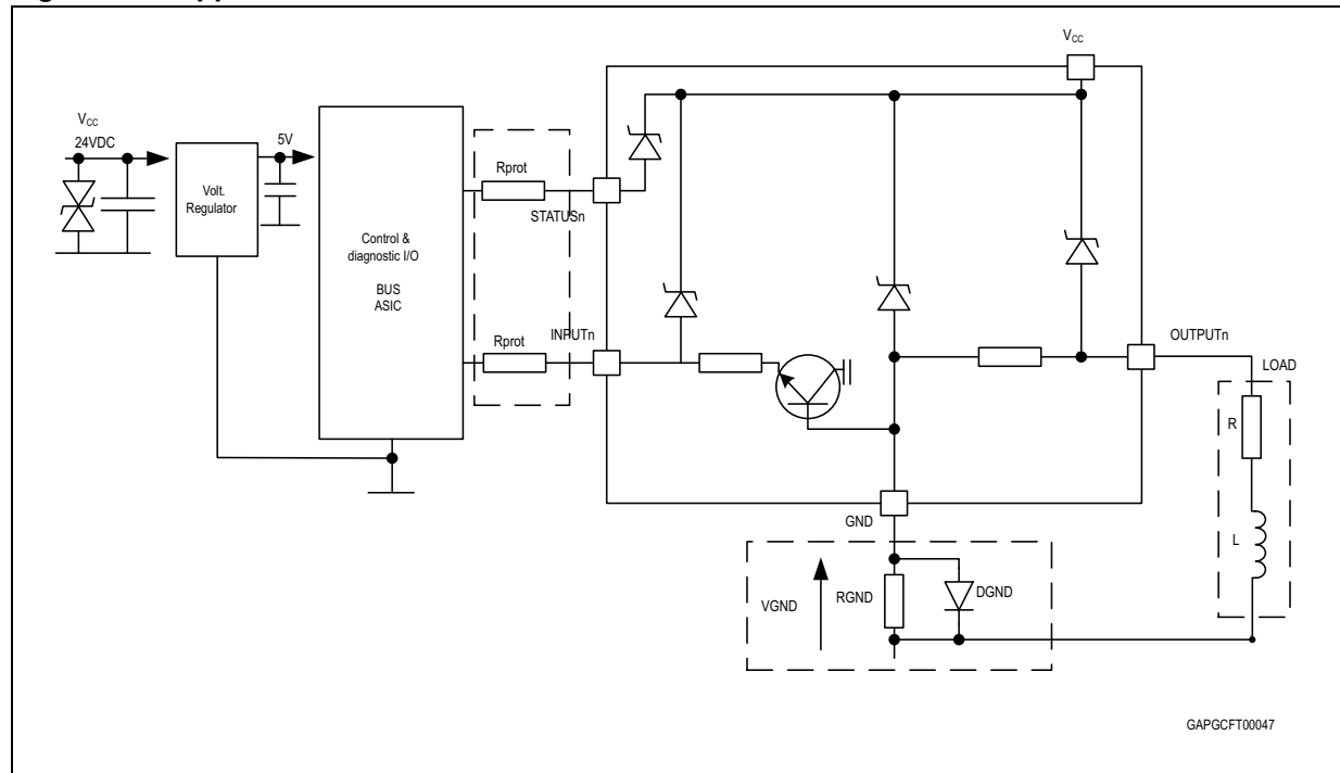
Figure 9. Application schematic
