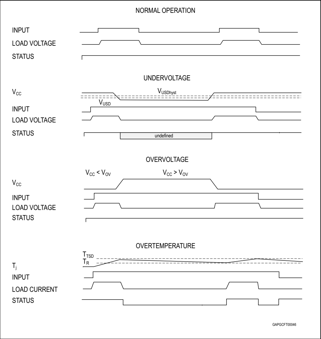
Figure 8. Waveforms
