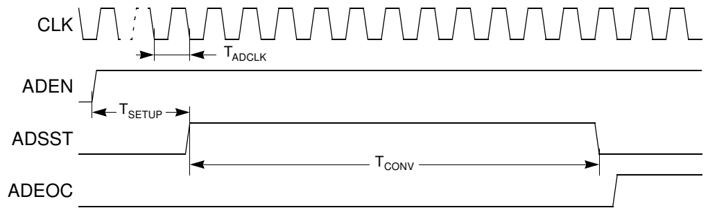
Figure 21-2. Timing Diagram
