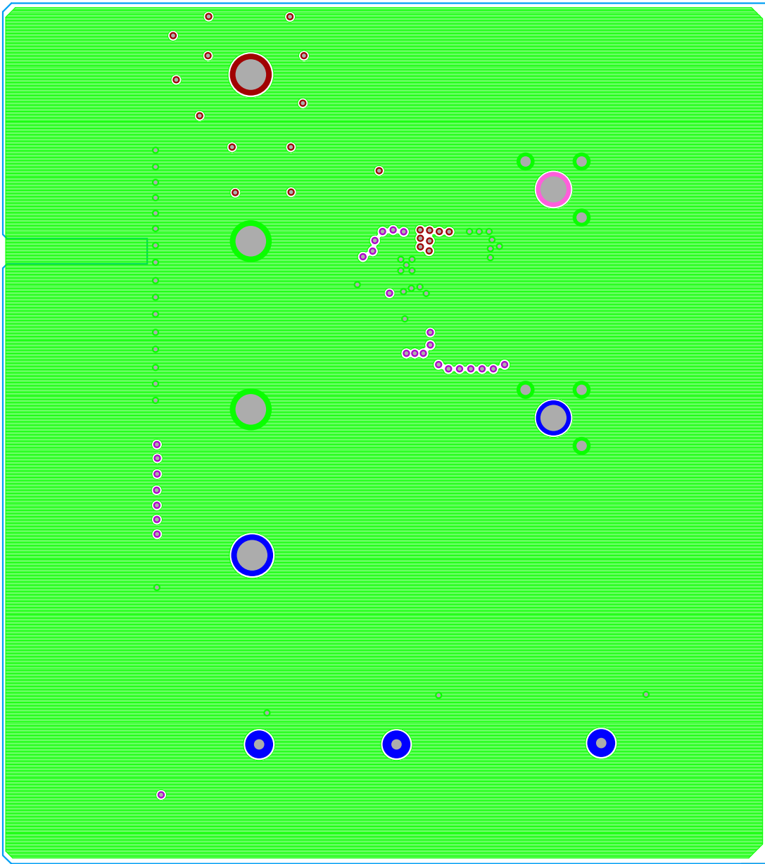
FIGURE 3. SECOND LAYER ETCH
