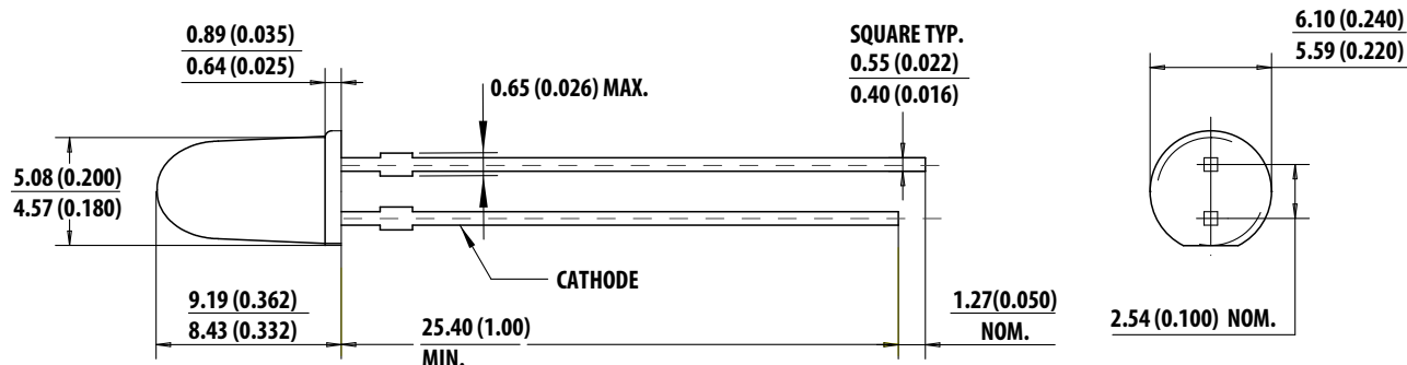
A - HLMP-4700, -4719, -4740
