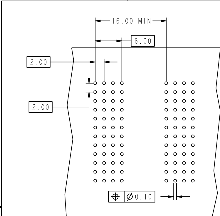
REQUIRED PC BOARD LAYOUT COMPONENT SIDE
