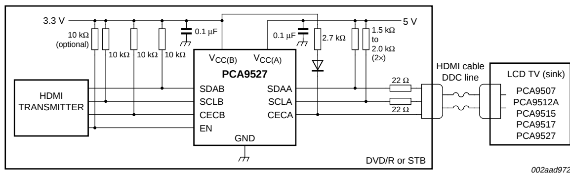
Fig 6. Source or DVD/R, STB application
