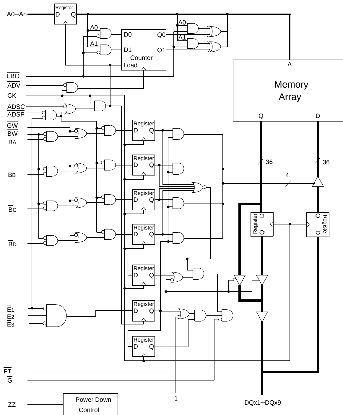
GS832118/32/36A Block Diagram
