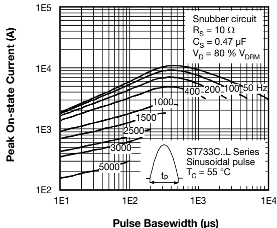
Fig. 13 - Frequency Characteristics
