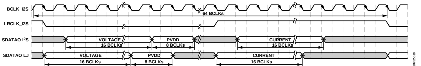
Figure 42. I²S and Left Justified Modes with Voltage, Current, and PVDD Output, 64 \times f_s
