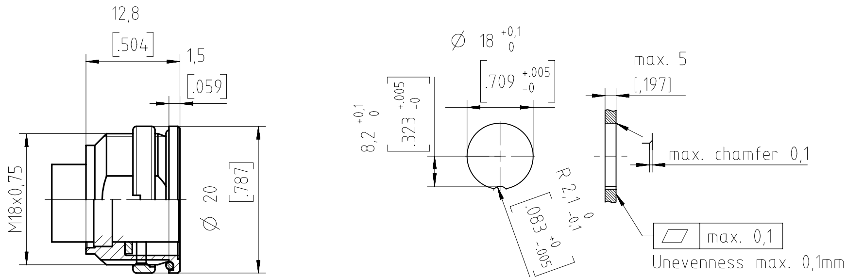
Panel Cutout M1:1
